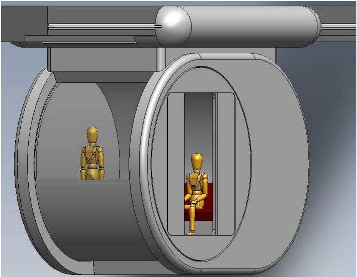
Figure 8 shows the lightweight “Skytrak” passenger cabin which can accommodate both standing and seated passengers as well as two curved windows for “scenic” applications
