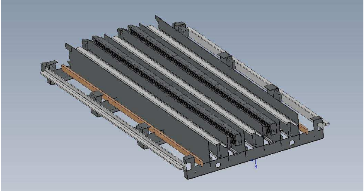
Figure 7 shows a possible arrangement of the track elements and structure to be built in 5m straight or curved sections
